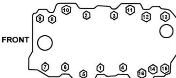
7620 & 7621 Torque Sequence
