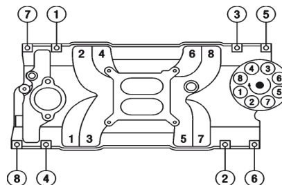
FIRING ORDER 1-8-4-3-6-5-7-2
