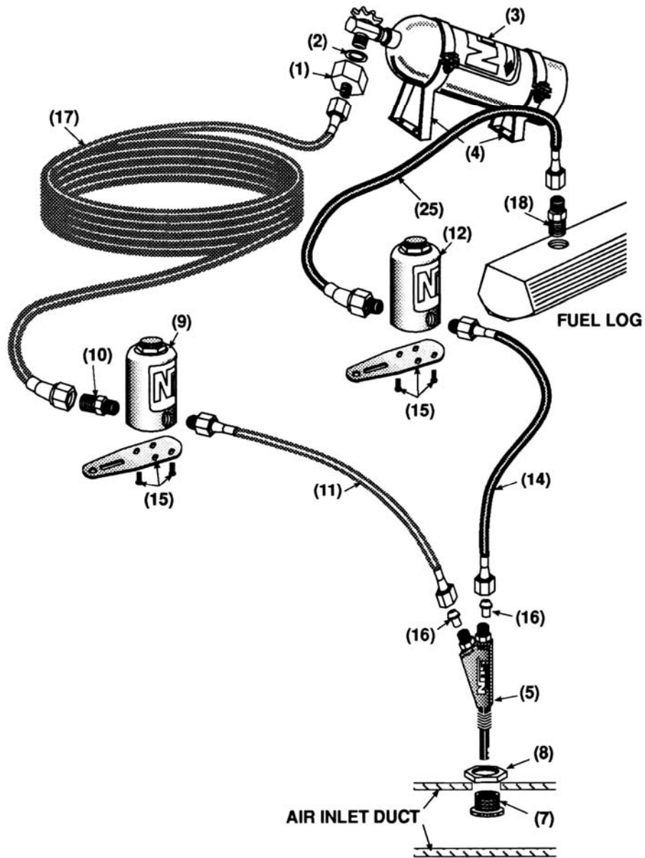
Figure 4 Exploded View of Factory Fuel Injection System
