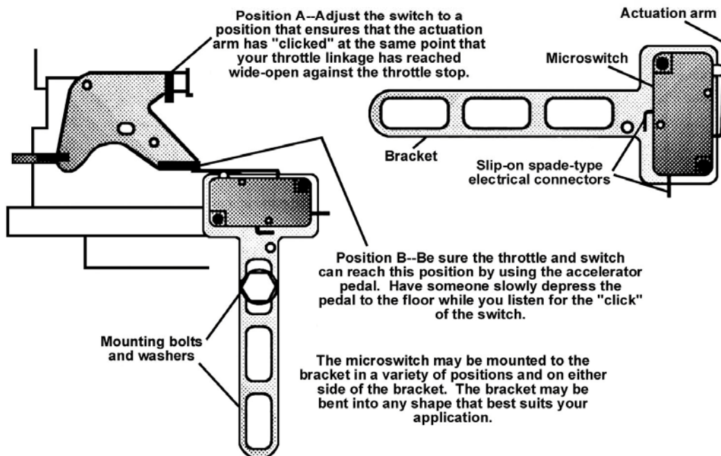
Figure 11 Microswitch Mounting
