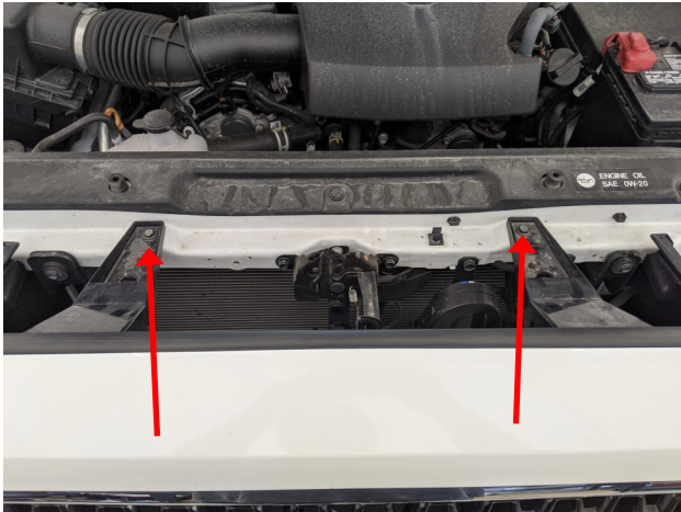
Figure 1a: Grille bolt locations
