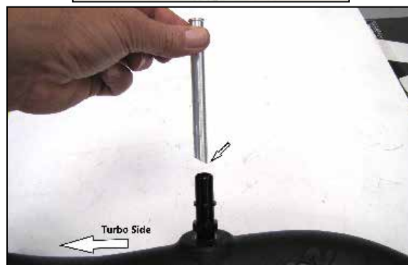
15. Install the CCV insert into the CCV fitting installed closest to the turbo side of the tube. Note the angle of the fitting, the short side is to be positioned towards the turbo. See photo.
