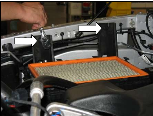
i. Remove the 2 bolts securing the air box base to the vehicle.
