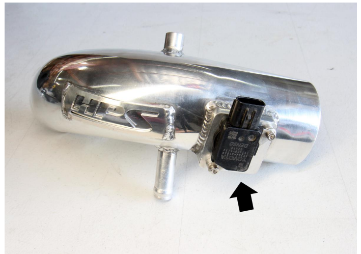
11. Transfer the MAF sensor from the stock air box onto the HPS intake pipe and secure it with the M4 screws provided.
