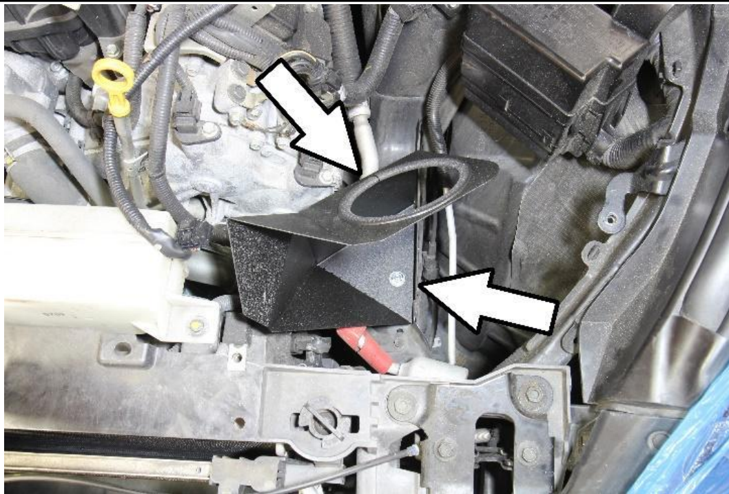
17. Install the thin edge trim onto the heat shield indicated above and secure the heat shield onto the bracket using a M6x12mm bolt and washer. Repeat this step on the passenger side.
