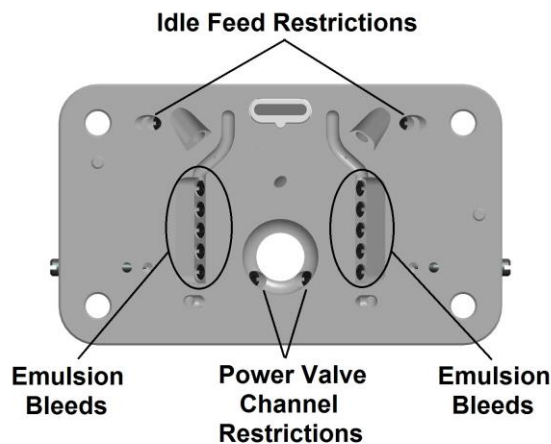
2 Circuit Billet Metering Block (Front) Model 4150 ALUMINUM XP Series Figure 6
