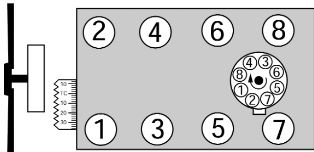
Figure 1 - 396-454 C.I.D. Chevrolet V8 Firing Order and Timing Marks
