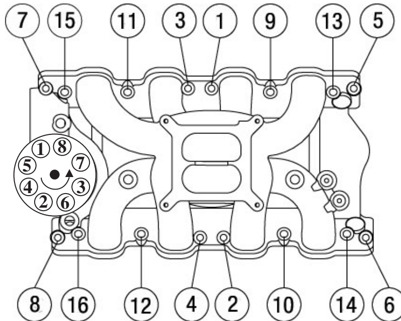
Figure 1 - 351C Ford Torque Sequence
