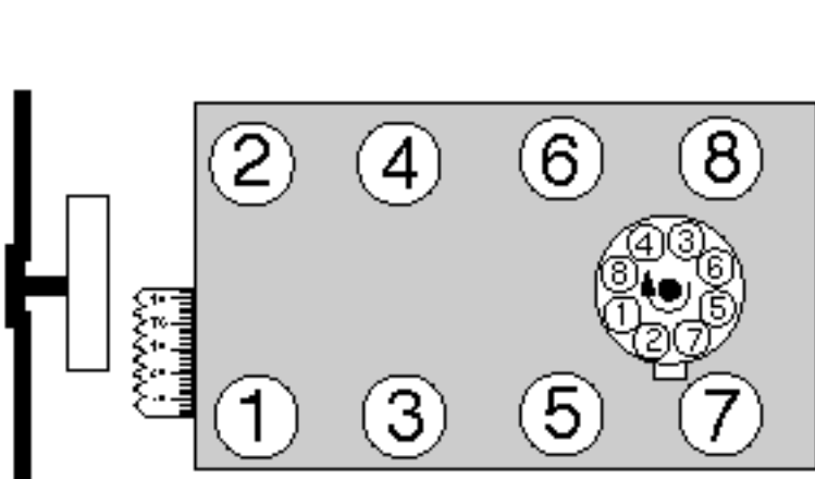
Figure 1- Chevrolet 265-400 c.i.d. V8 Firing Order 1-8-4-3-6-5-7-2 Turn distributor counter-clockwise to advance timing.
