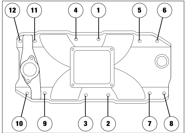
Figure 1 - 396-502 C.I.D. Chevrolet Bolt Torque Sequence Torque Bolts To 25 ft./lbs.
