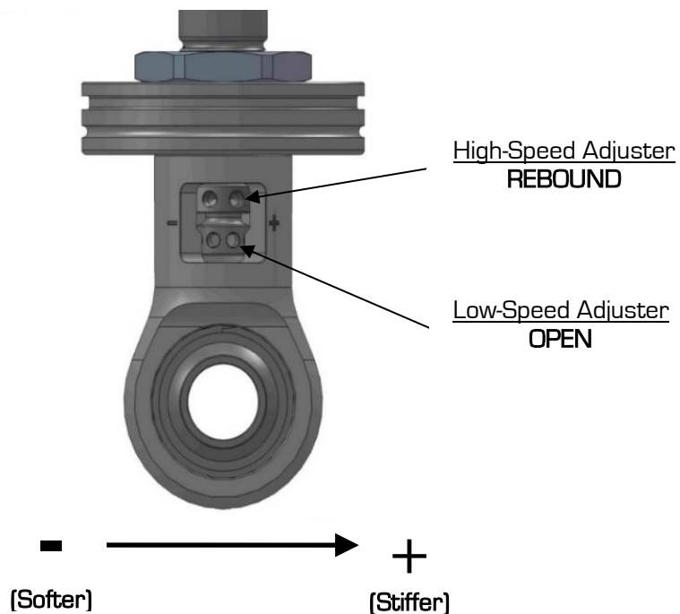
Figure 41b – Detroit Speed Recommended Settings
