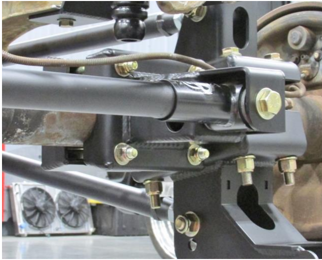
Figure 29 – Install Track Bar
