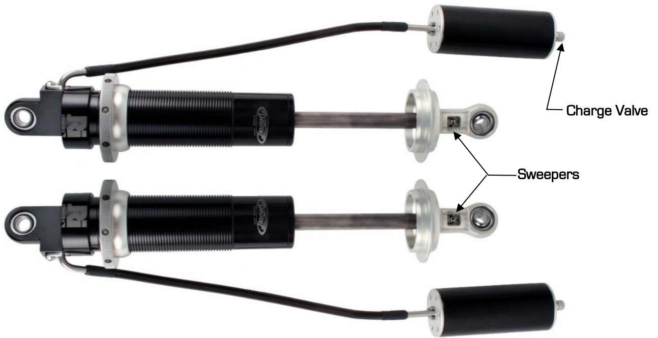
Figure 41a – Detroit Speed Double Adjustable Shock w/ Remote Canister
