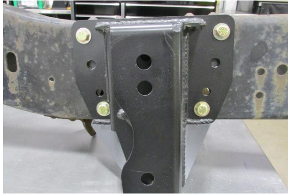
Figure 18 - Locate Mounting Holes
