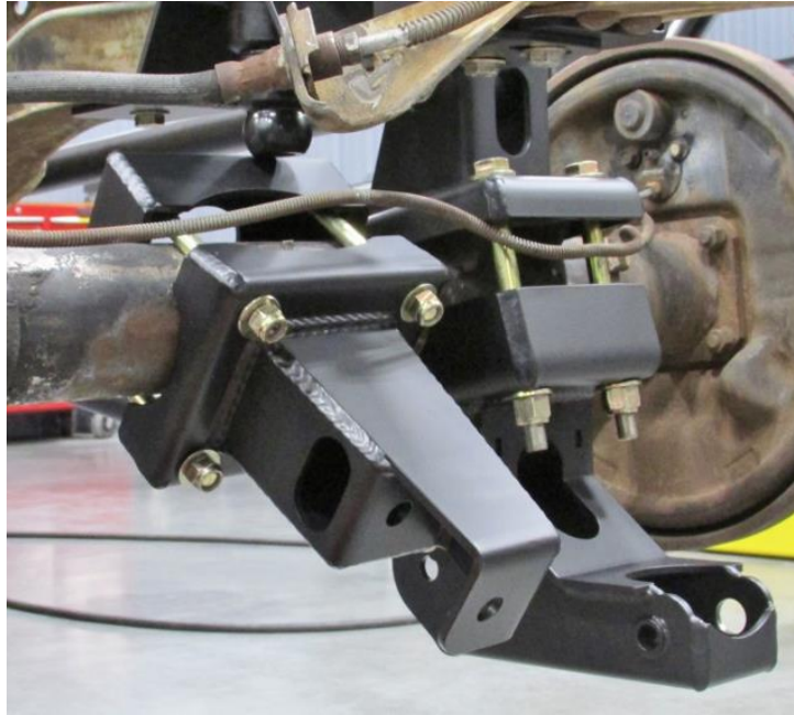
Figure 26 – Position Track Bar Axle Bracket
