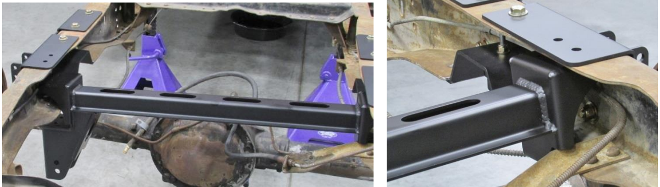
Figure 13 - Position Crossmember Assembly
