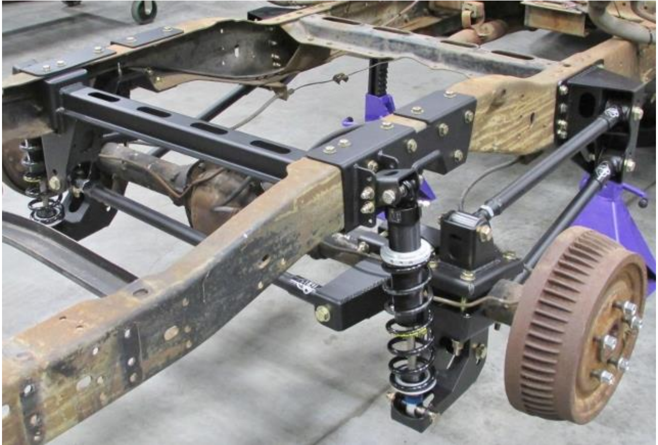
Figure 38 - Final Assembly
