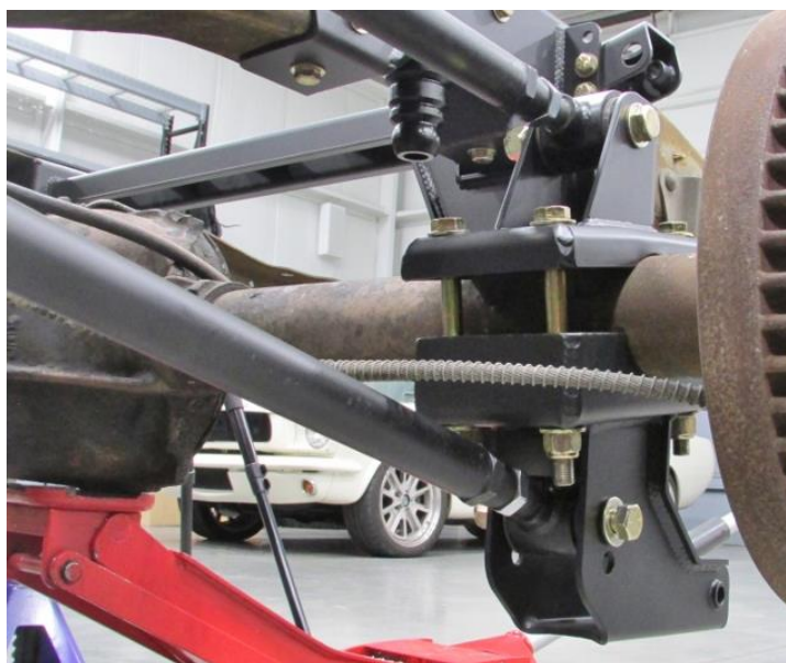
Figure 25 - Install Links to Axle Brackets (PN: 041750 Shown)
