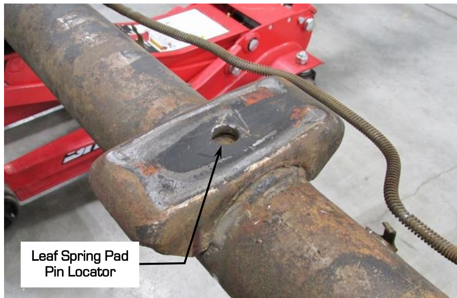
Figure 22 – Factory Leaf Spring Pad
