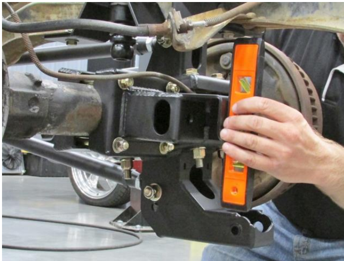
Figure 27 – Level Track Bar Axle Bracket
