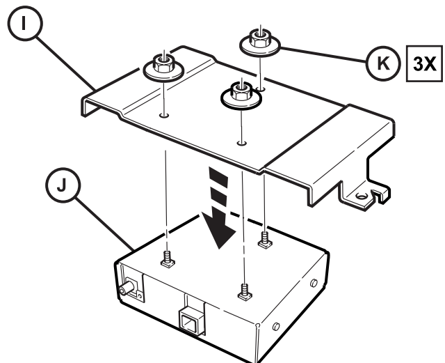
29 Assemble bracket to receiver.
