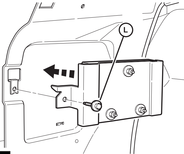
30 Install receiver assembly.
