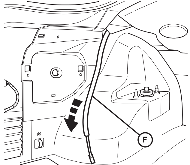
27 Route extension cable into trunk.
