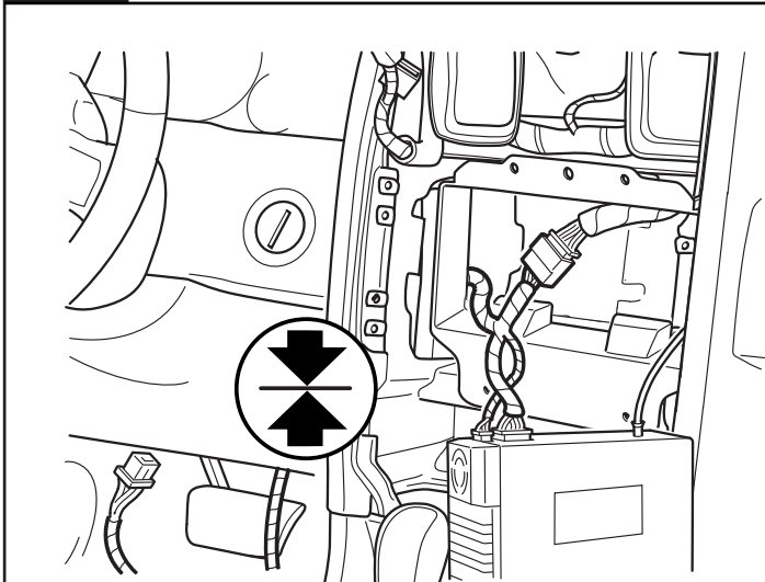
11 Disconnect 22-way radio connector. Plug harness connectors in-between.
