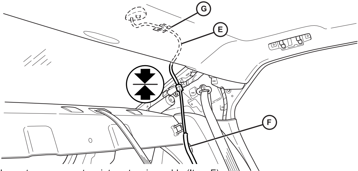
25 Plug antenna connectors into extension cable (Item F)
