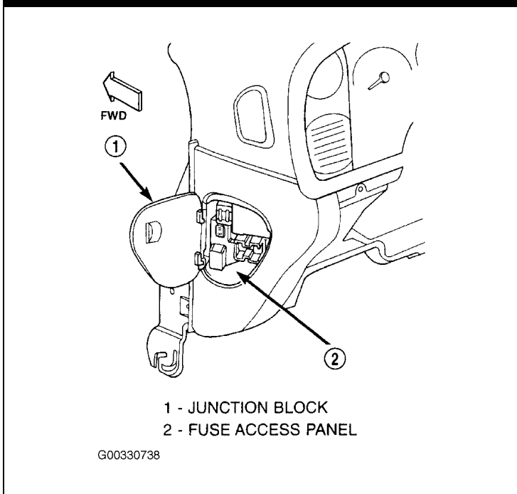
Fuse # 2 (10 Amp)
