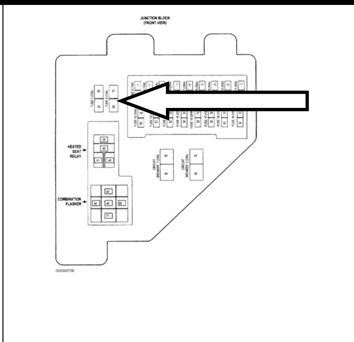
Fuse # 2 (10 Amp)
