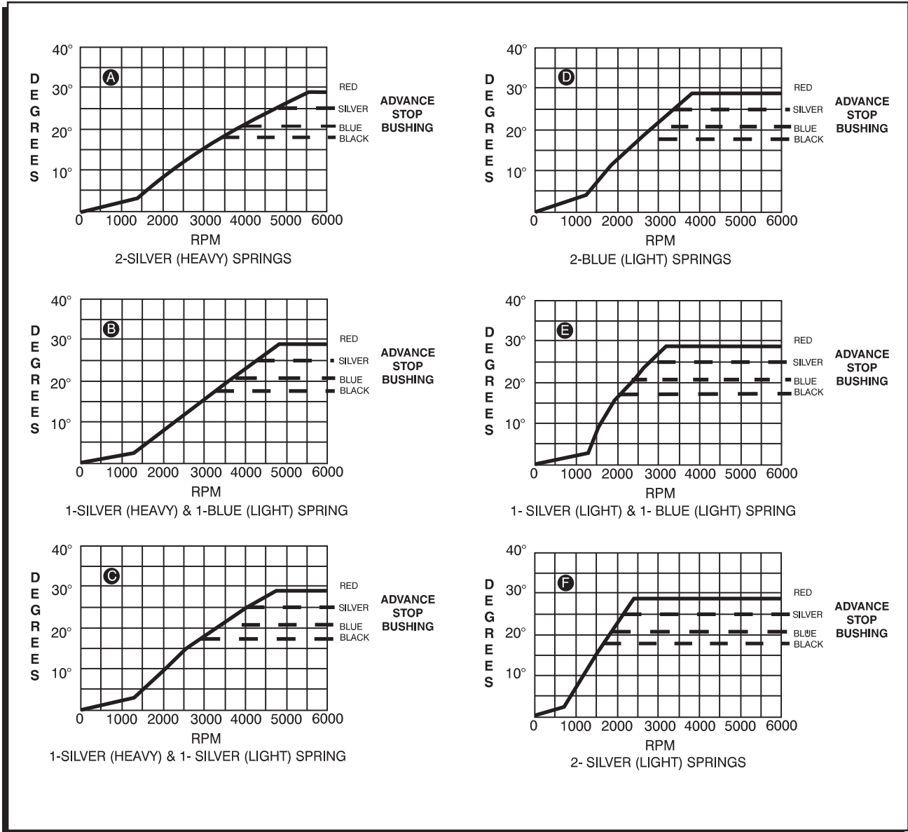
Figure 3 Advance Curves.
