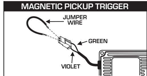
Figure 10 Checking for Spark with Magnetic Pickup.
