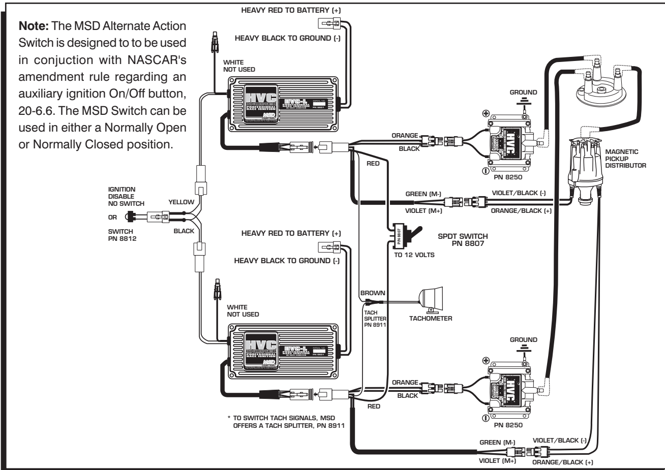
Figure 3 Dual Ignitions and Coils with a Dual Pickup Distributor.
