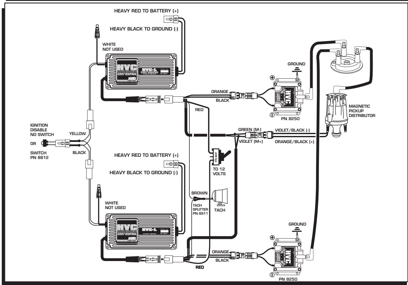
Figure 4 Dual Ignitions and Coils with a Single Pickup Distributor.
