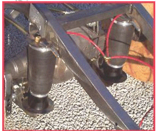
Rear "pro street" installation [fully extended]
