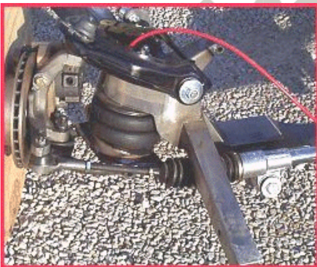
Mustang II front end fully compressed
