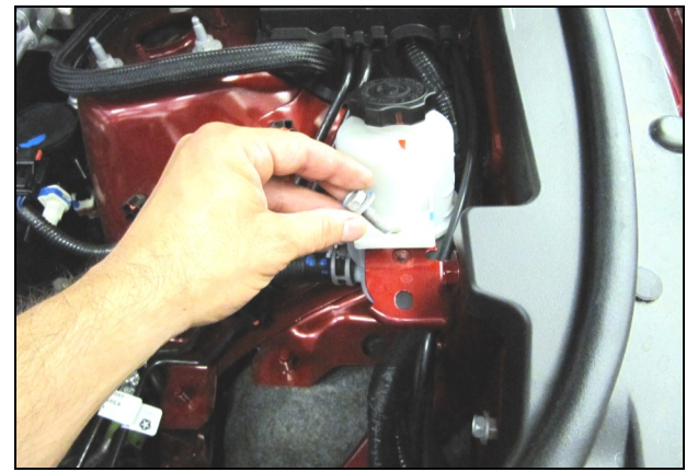
12. Remove the bolt securing the power steering reservoir and set it aside. This bolt will be reused in step 13. to hold the Mounting bracket.
