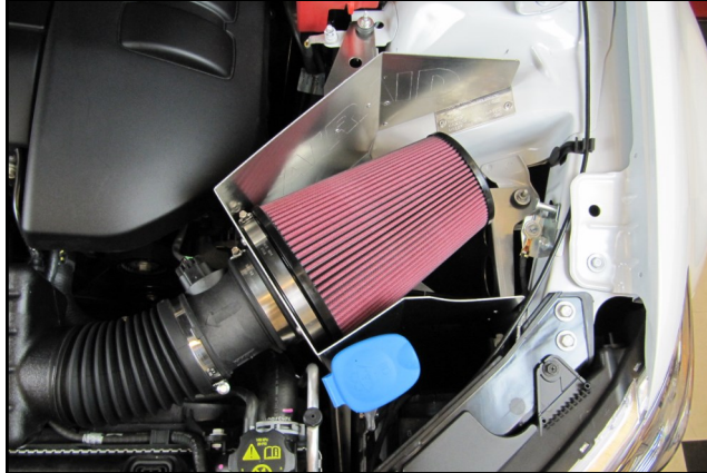
14. Install the Airaid Premium Filter on to the Filter Adapter.
