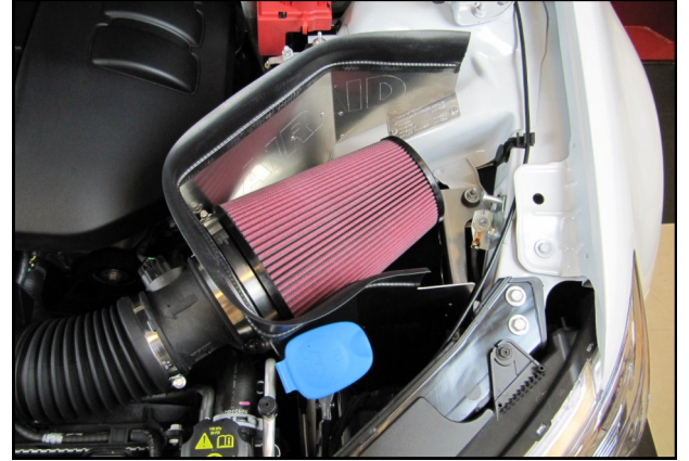
15. Install the Weatherstrip onto the top edge of the Air Dam with the contour rolling away from the Filter.
