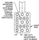
FOOT PAD DETAIL
