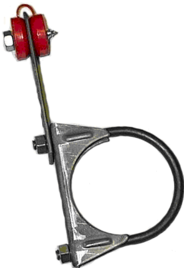
Rear tail pipe hanger assembly
